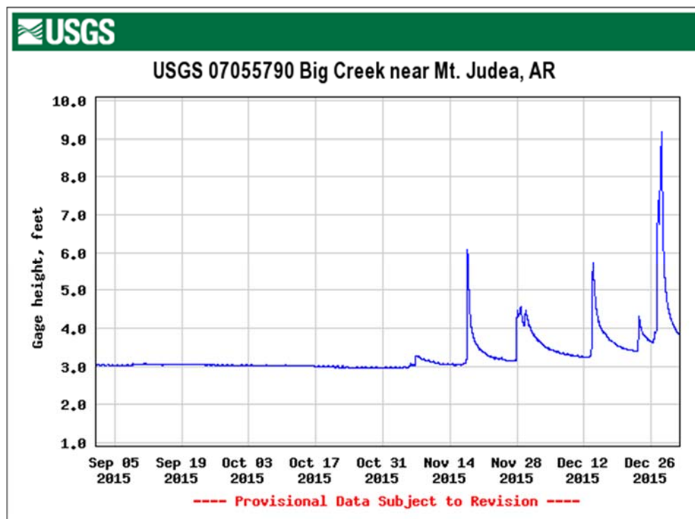
Figure 1. Gage height at the Big Creek monitoring site downstream of the C&H Farm during the 4 th quarter of 2015.
