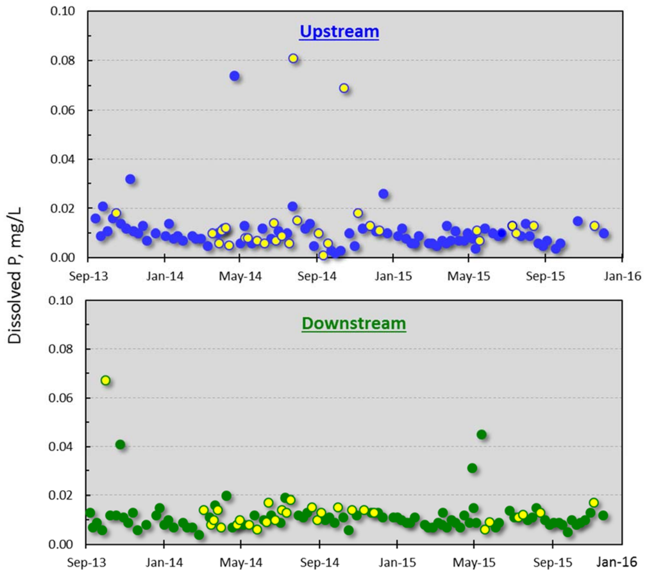
Figure 5. Dissolved P concentration at the Big Creek monitoring site up- and downstream of the C&H Farm, Newton County, AR.
