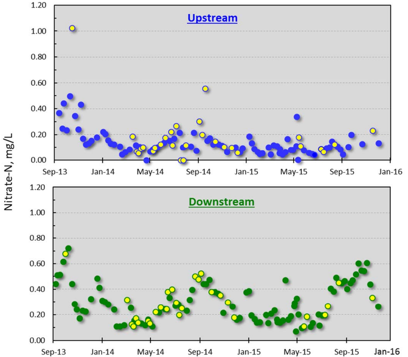
Figure 7. Nitrate-N concentration at the Big Creek monitoring site up- and downstream of the C&H Farm, Newton County, AR.
