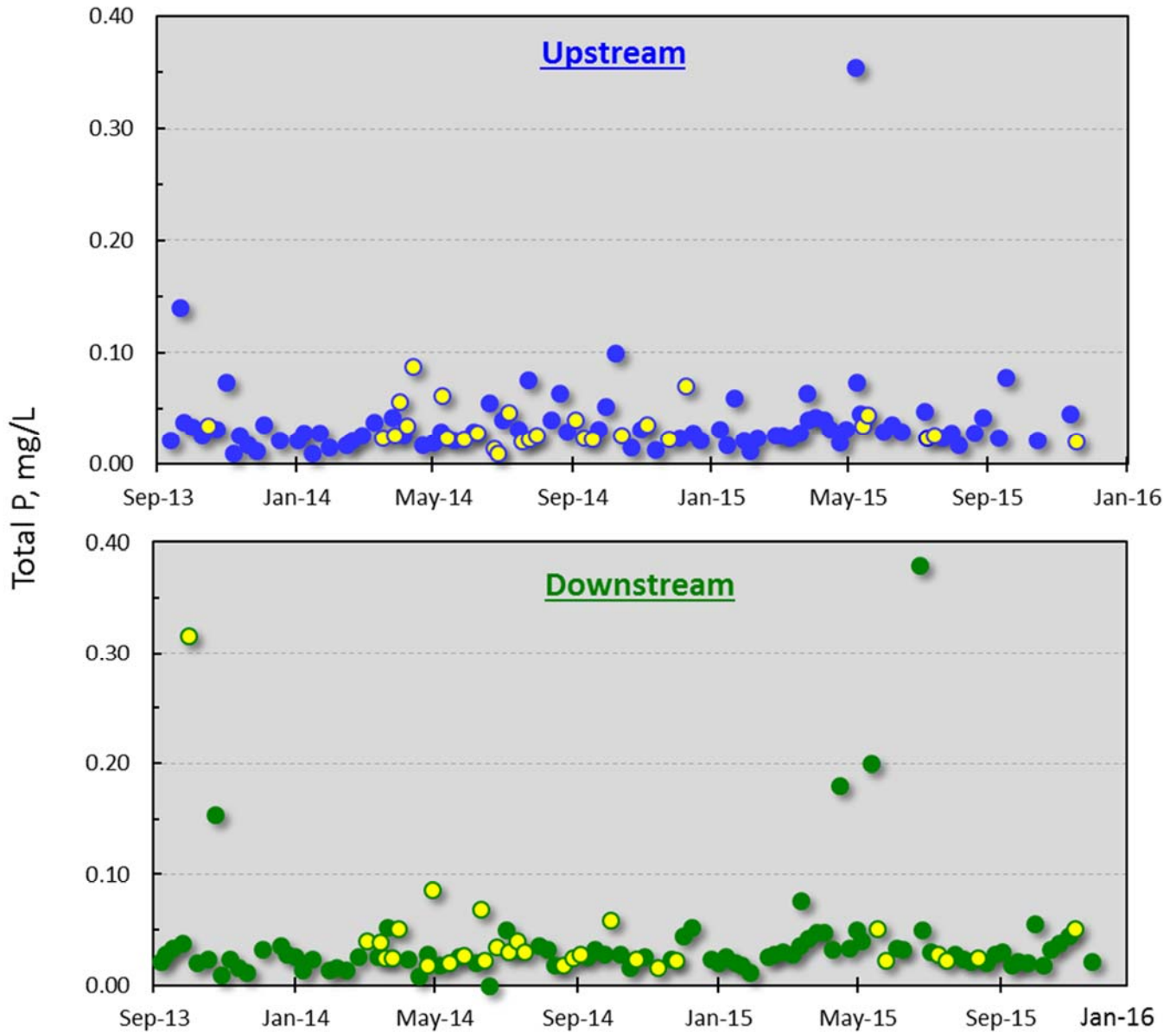
Figure 6. Total P concentration at the Big Creek monitoring site up- and downstream of the C&H Farm, Newton County, AR.
