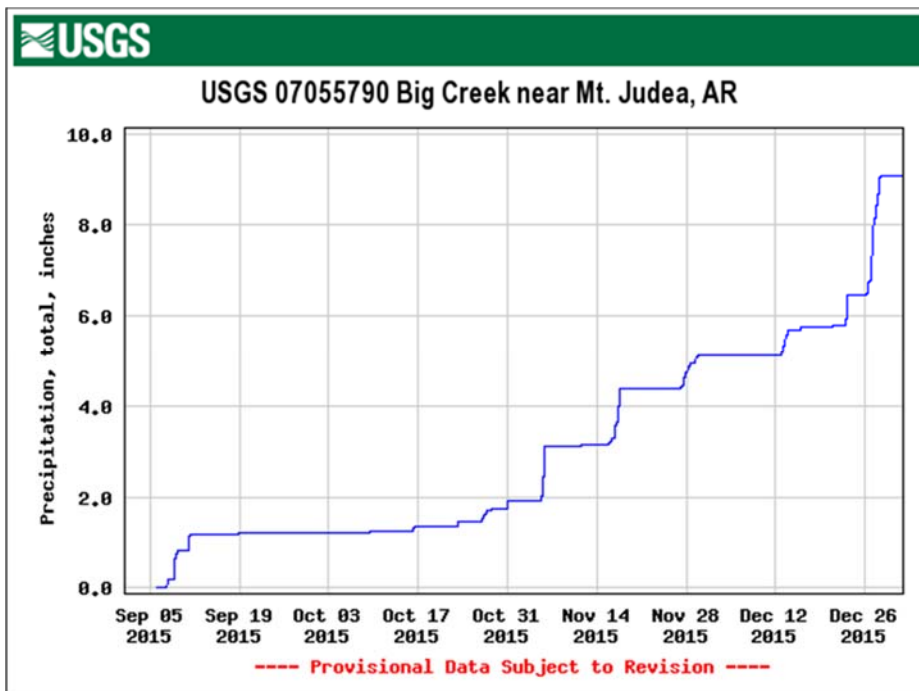
Figure 3. Precipitation at the Big Creek monitoring site downstream of the C&H Farm during the 4 th quarter of 2015.
