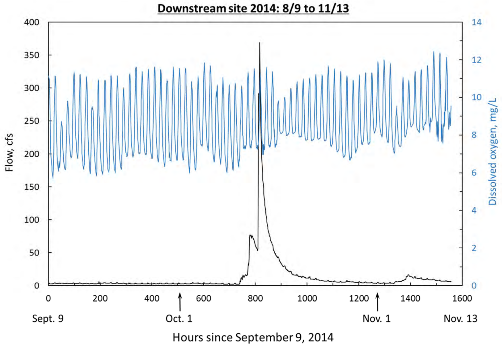
Figure 2. Flow and dissolved oxygen concentration downstream of the C&H Farm between September 9 and November 13, 2014.
