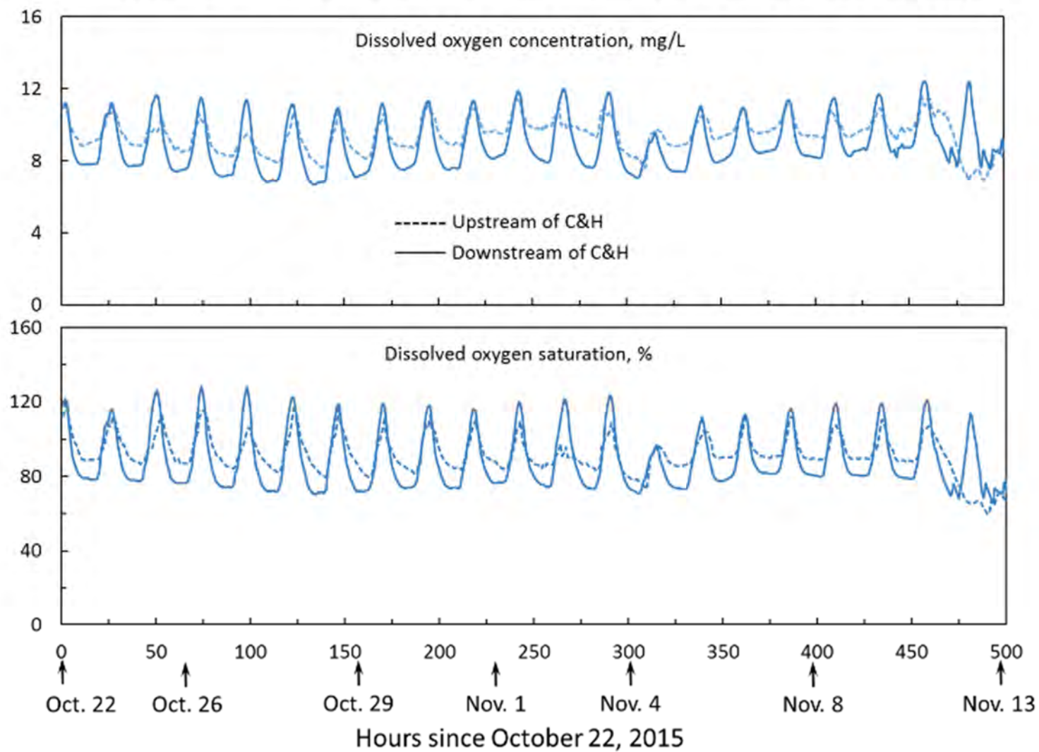
Figure 18. Dissolved oxygen concentration and percent saturation upstream and downstream of the C&H Farm between October 22, 2014 and November 13, 2014.
